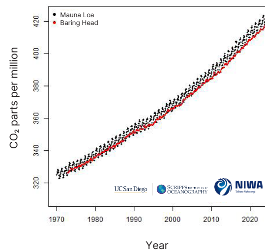
Mauna Loa and Baring Head CO 2
